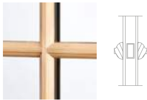
COLONIAL SIMULATED DIVIDED LITES
